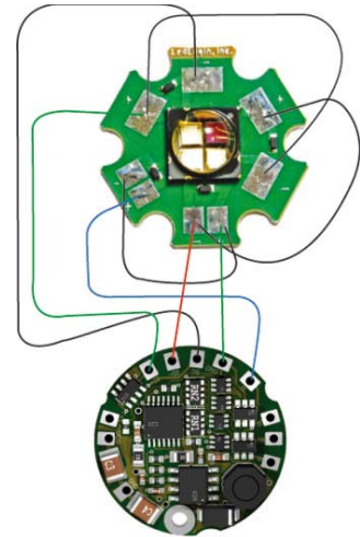
Sample wiring schematic of L-Dot Pico with LedEngine 10W RGB
